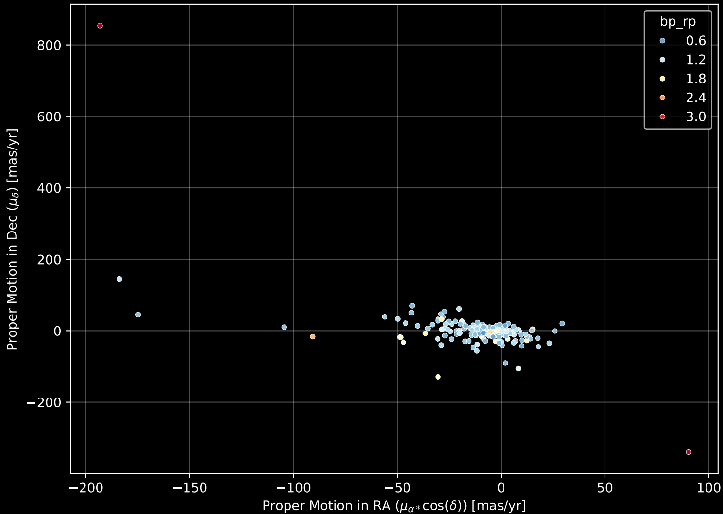
APOGEE DR17 Field: [058+44_MGA] Proper Motion Diagram (n= 197)
