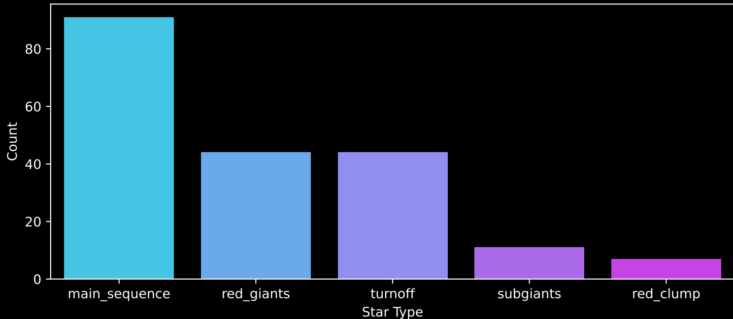
APOGEE DR17 Field: [058+44_MGA] Count plot of Star Type
