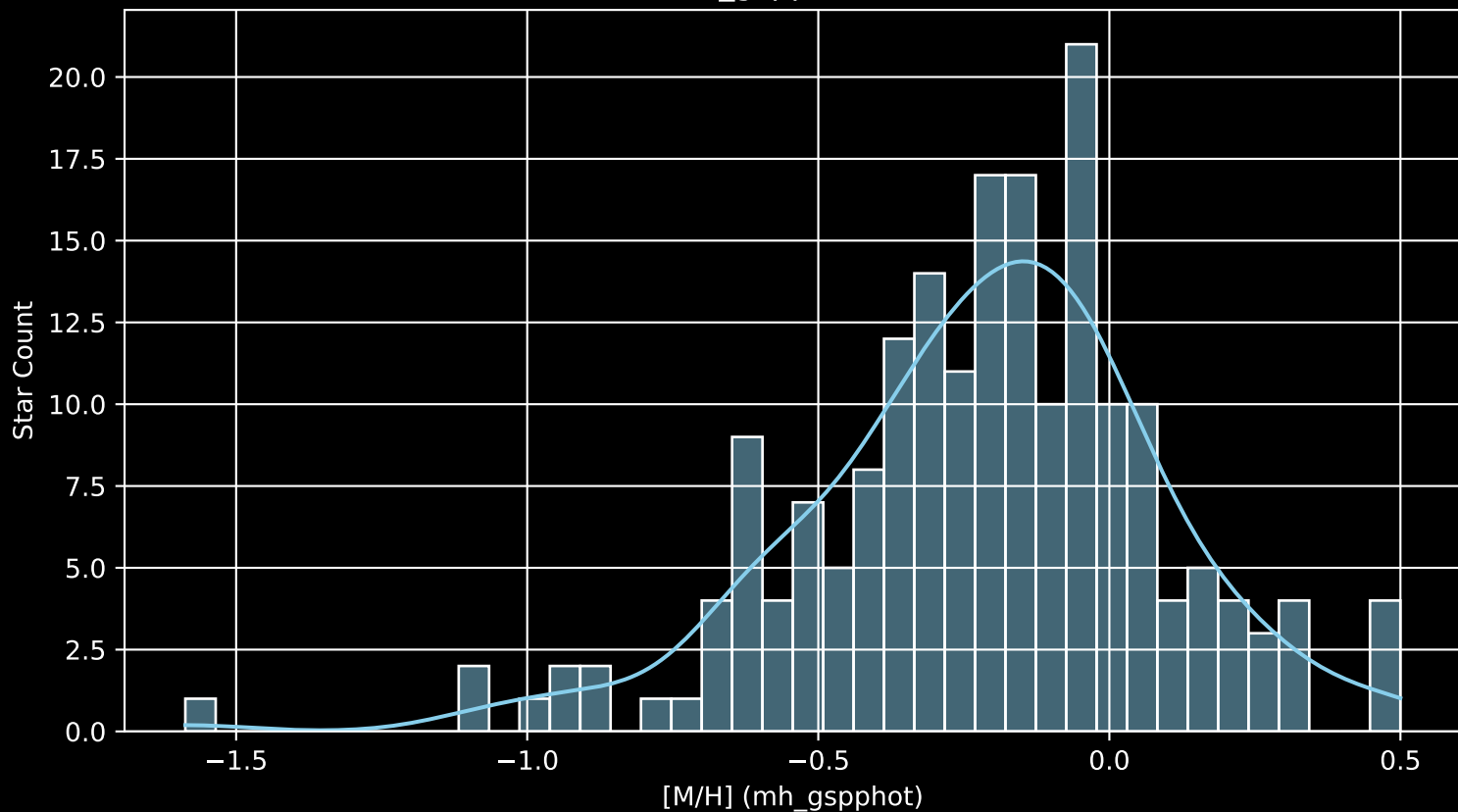
APOGEE DR17 Field: [058+44_MGA [M/H] (mh_gspphot) (n= 193)
