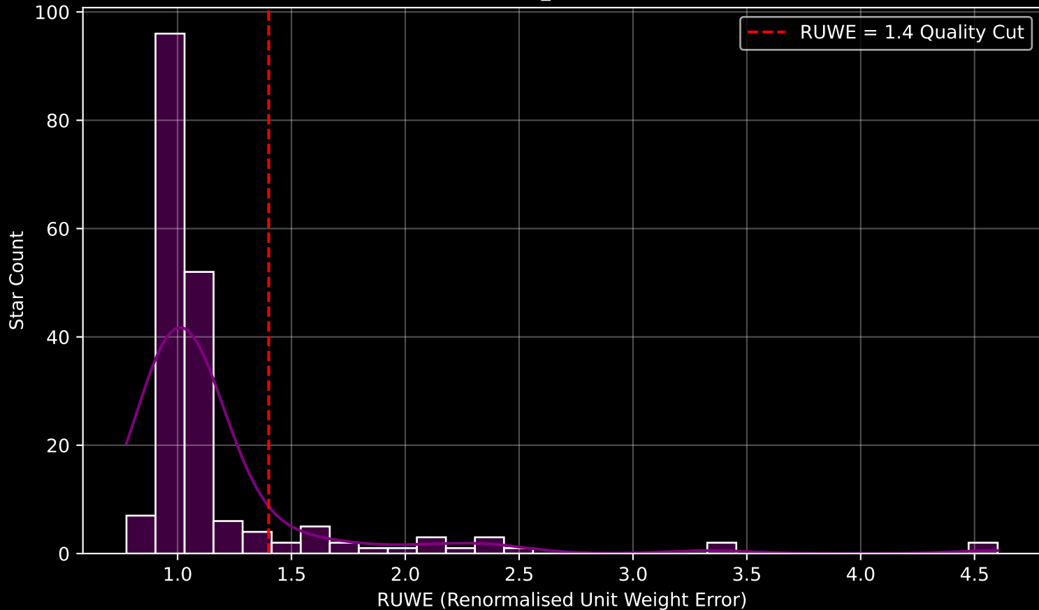
GAPOGEE DR17 Field [058+44_MGA] RUWE Distribution (n= 188)
