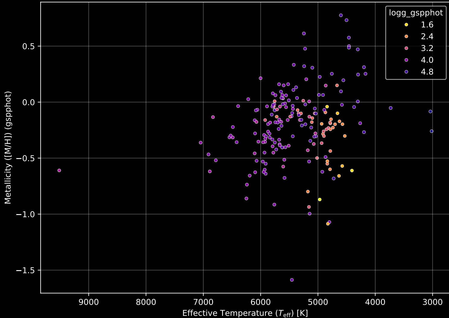
APOGEE DR17 Field: [058+44_MGA] Stellar Population Parameters (n= 197)
