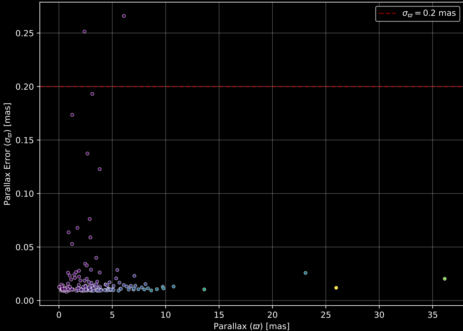
APOGEE DR17 Field: [058+44_MGA] Parallax Quality (n= 197)
